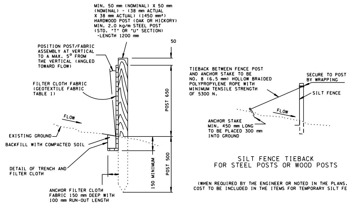
SECTIONAL VIEW
